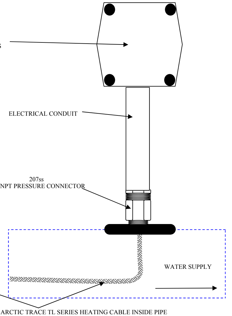
208C NEMA 4X JUNCTION BOX WITH DIN RAIL TERMINALS
