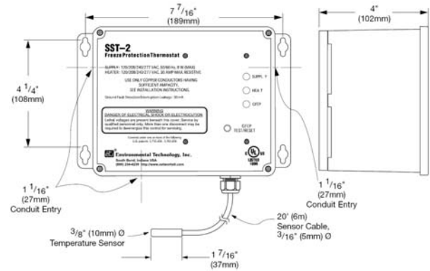
SST-2 DIGITAL THERMOSTAT
